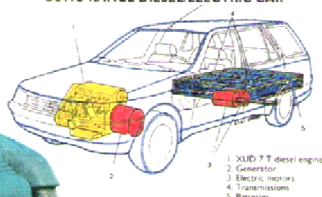
PEUGEOT 405 STATION WAGON: LONG-RANGE DIESEL/ELECTRIC CAR
