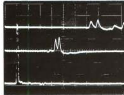
Figure 8: Signal on passive right line with its front end shorted to ground
