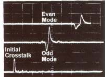
Figure 3b: Signal on passive right hand line.
