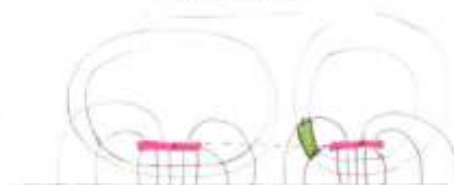
Figure 9: Field patterns for Even Mode and Odd Mode for surface lines. It is simpler to think of four conductors rather than two conductors and a ground plane
